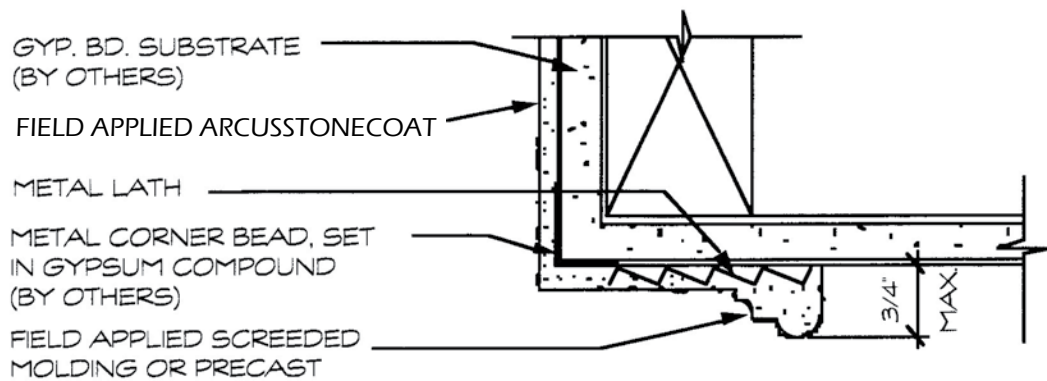
TYP. SCREEDED MOLDING @ CASED OPENING
