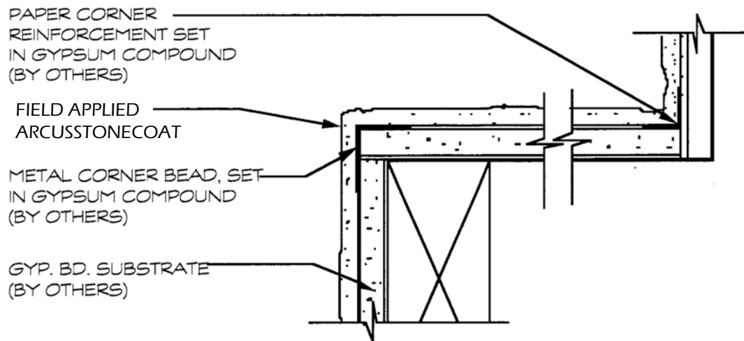
TYPICAL CORNERS
