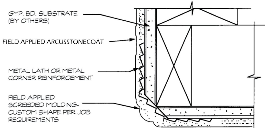
TYPICAL SCREEDED MOLDING @ OUTSIDE CORNER
